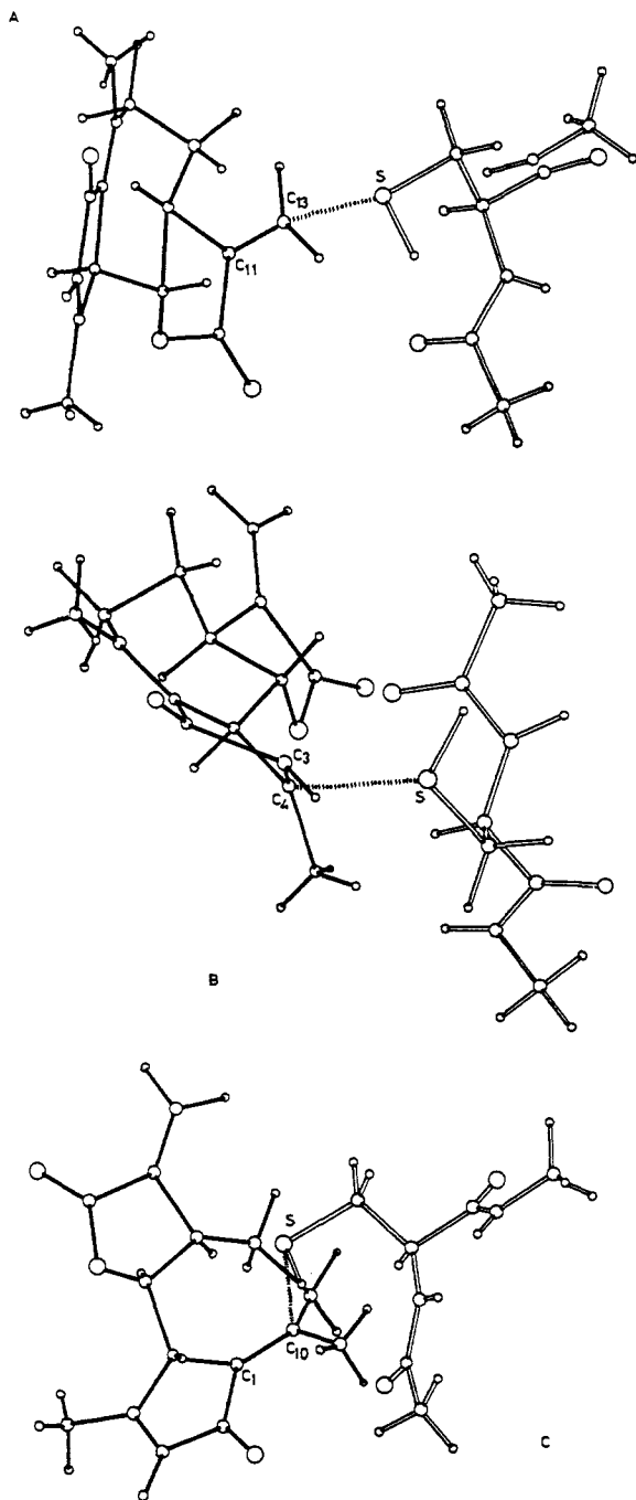
Figure 1. Spatial view of the intermolecular interactions between the chair form of dehydroleucodin (1) and a blockable cysteine residue. (A) Interaction with C 11 -C 13 double bond; (B) interaction with C 3 -C 4 double bond; (C) interaction with C 10 -C 1 double bond.
