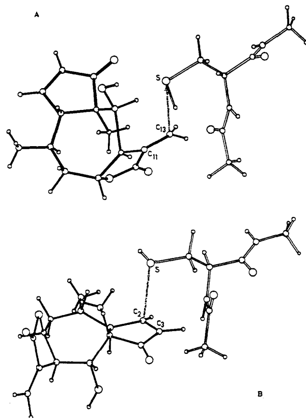
Figure 3. Spatial view of the intermolecular interactions between the chair form of helenalin (2) and a blockable cysteine residue. (A) Interaction with C 11 -C 13 double bond; (B) interaction with C 2 -C 3 double bond.
