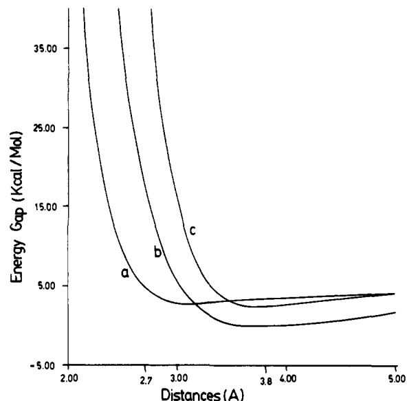
Figure 2. Energy profiles for the intermolecular interaction between the chair form of dehydroleucodin (1) and a blockable cysteine residue. (a) Cysteine-C 11 C 13 double bond; (b) cysteine-C 3 C 4 double bond; (c) cysteine-C 10 C 1 double bond.
